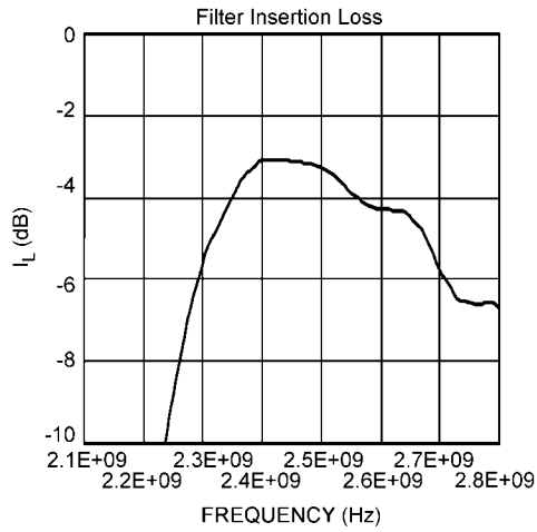
20180050 Front-End Bandpass Filter Response
