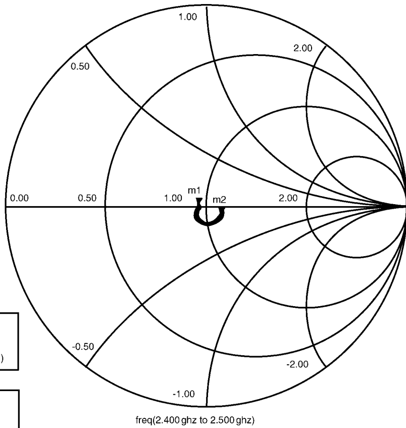
20180050 Front-End Bandpass Filter Response
